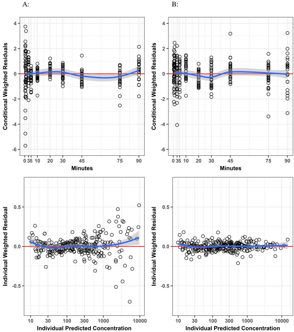
Supplemental Figure 1: Comparison of Goodness-of-Fit Plots for a 3- (A) and 4- (B) Compartment Model
