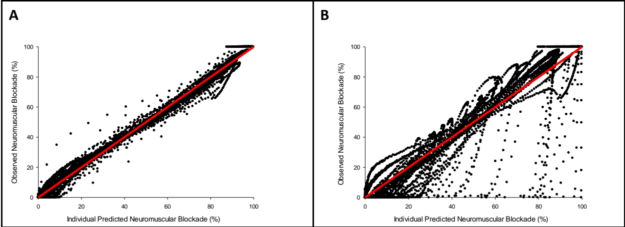
Supplemental Figure 7: Goodness-of-Fit Plots for PK-PD Model. Transit Compartment Model (A) and Basic Effect Compartment Model (B)
