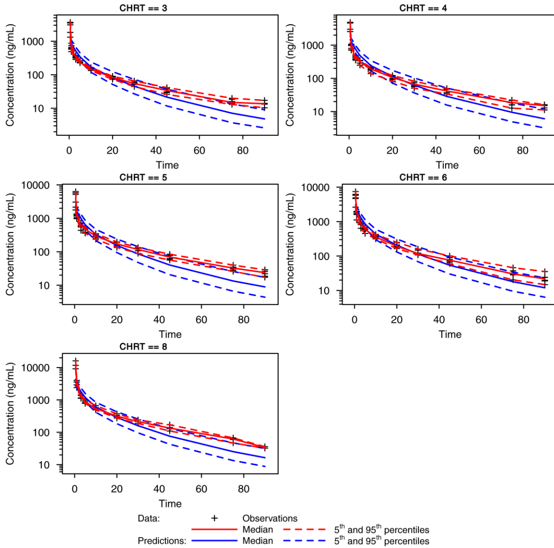
Supplemental Figure 6: Visual Predictive Check for 3-Compartment Fixed Plasma Volume PK Model by Cohort (Semi-logarithmic scale)
