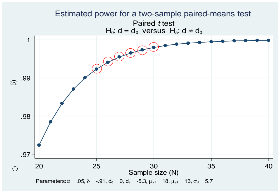
eFIGURE 2. Sample size calculation.
