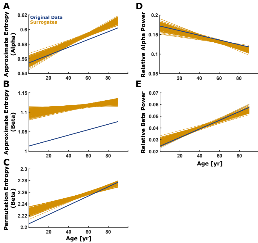
Figure S6: Results from the phase-randomized surrogate analysis of the parameter settings showing significant changes with age, i.e., for the approximate entropy in the alpha- (A) and beta-band (B), the permutation entropy in the beta-band (C), as well as for the relative alpha- (D) and beta-band power (E).
