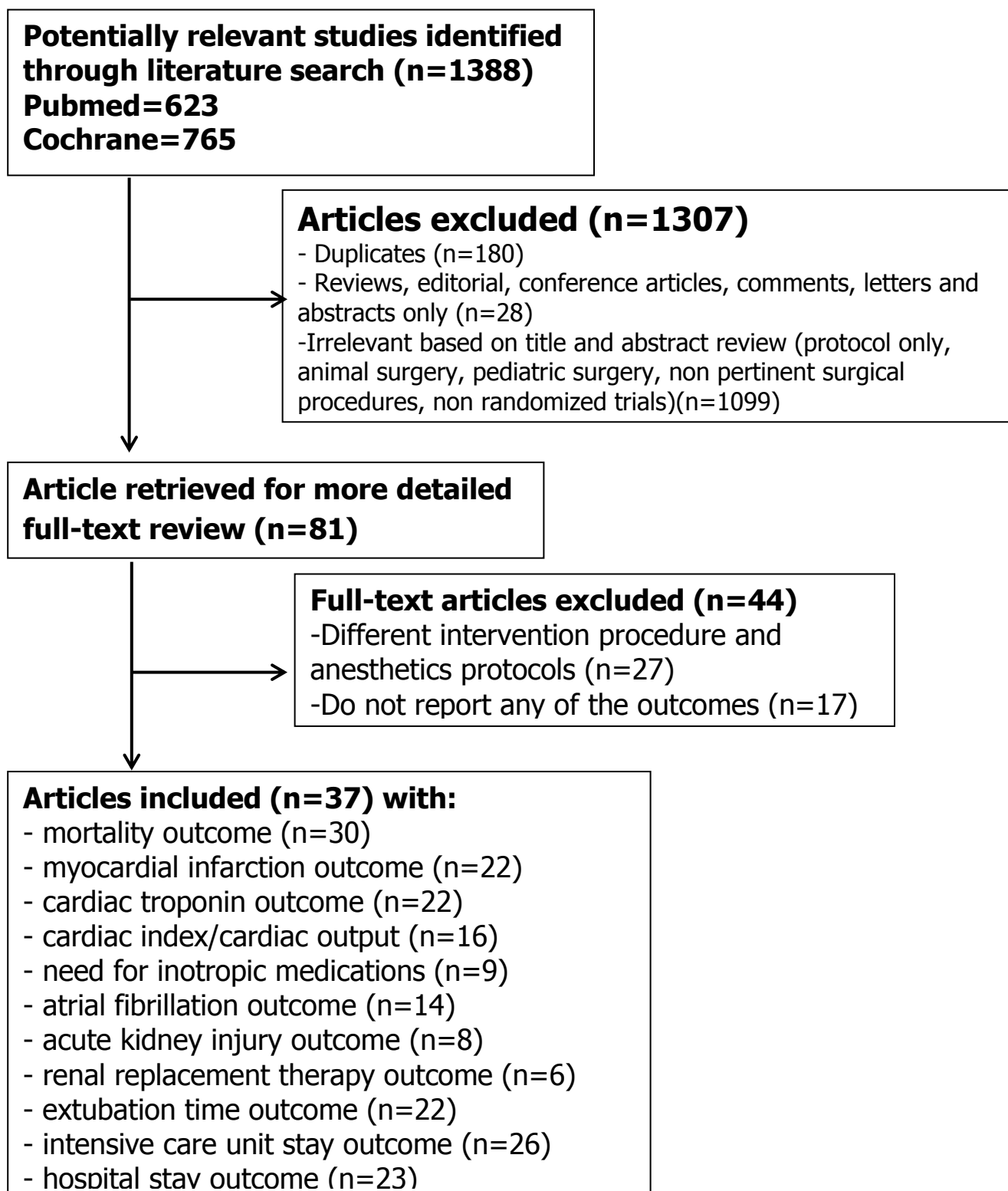
Figure 1: Flow chart of the search of studies for meta-analysis
