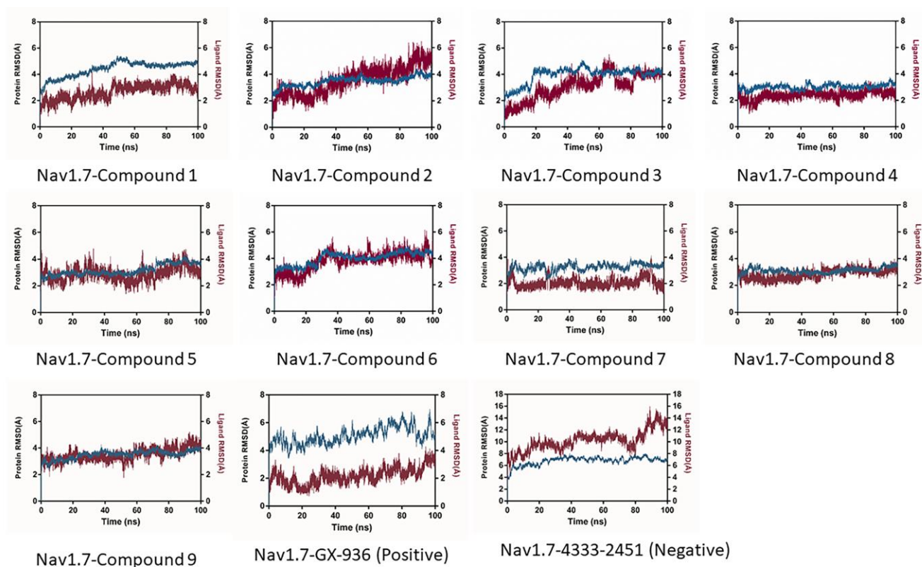
Supplementary Figure S1: Graphs of Root Mean Square Deviation (RMSD) of protein backbones (shown in blue lines) and ligand heavy atoms (shown in maroon lines) for identified compounds and controls. We have investigated the RMSD to measure the average change in displacement of atoms for a particular frame with respect to a reference frame.
