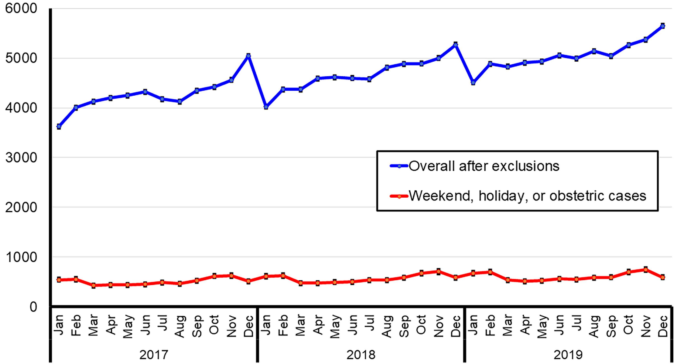
Appendix Figure 1: Daily caseload by month both overall after exclusions and weekend, holiday and OB cases. “Overall after exclusions” data plotted as total cases per month divided by number of working days in that month. “Weekend, holiday, and obstetric cases” data plotted as total cases per month divided by the total number of days in that month. Error bars: population 95% confidence interval
