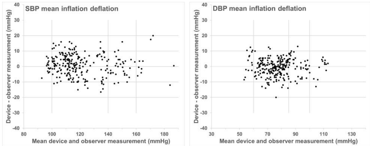
Figure S 1: Bland-Altman scatterplots of mean ABPMpro (mean calculation of inflation and deflation) and observer measurements for SBP (left) and DBP (right) (general validation study).
