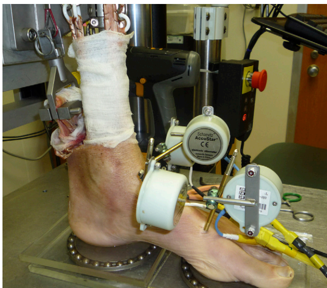
Fig. E-1 Medial view of a specimen in the testing machine. The hindfoot and forefoot rested on separate bearings to permit unrestricted motion of the sole relative to the table, while ankle flexion was maintained at 90°. Clinometers aligned in the sagittal plane measured talus-first metatarsal angulation, and those oriented in the coronal plane measured varus-valgus motion of the navicular in relation to the talus. The Achilles tendon clamp is visible posterior to tibial and fibular shafts.
