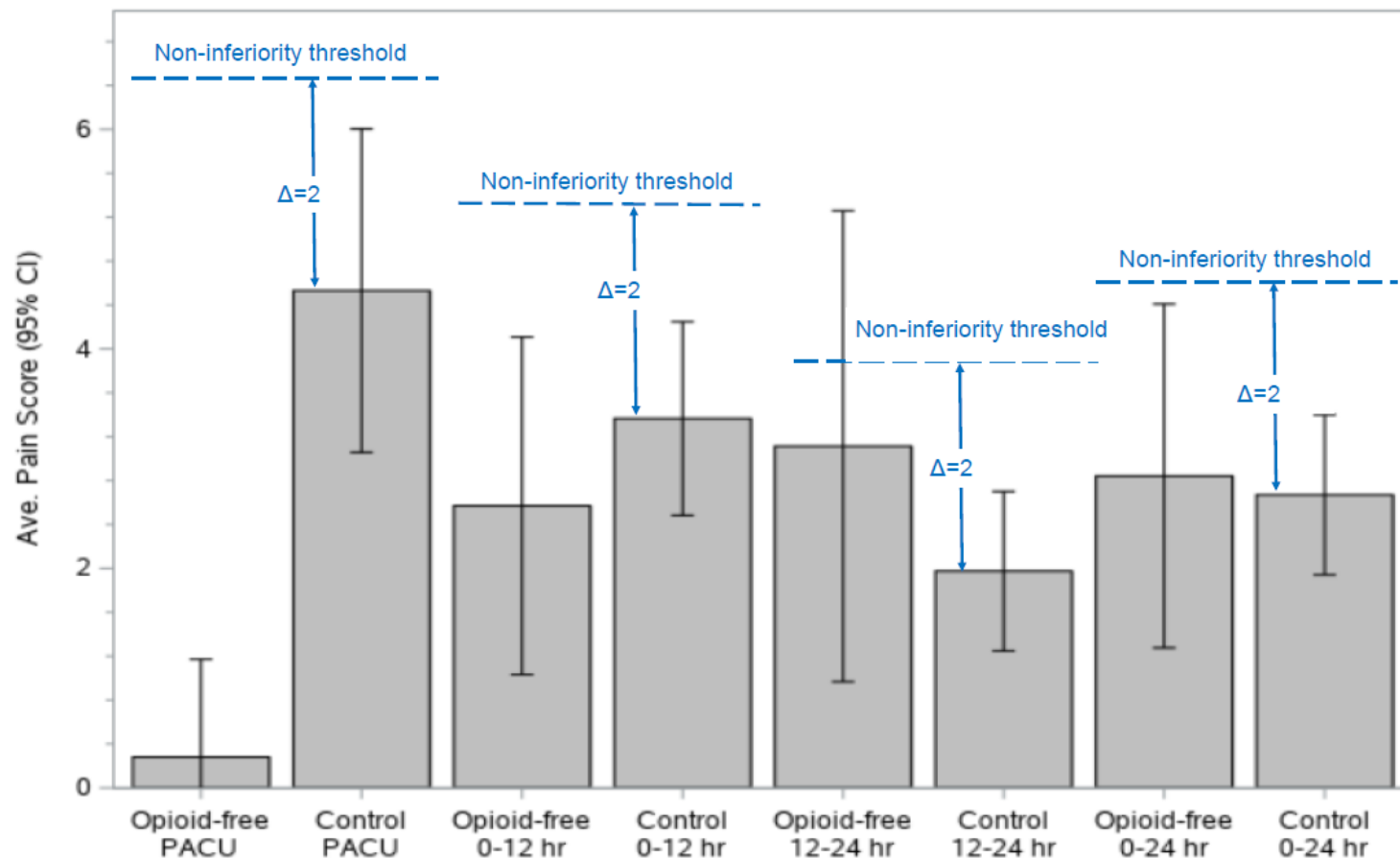
Supplemental Figure 2: Average pain scores for opioid-free vs. control group at overlapping time intervals. Since the upper confidence limit is below the Noninferiority Threshold (Control mean + preset noninferiority margin \Delta ), non-inferiority has been shown for pain for all time intervals except 12-24 h.
