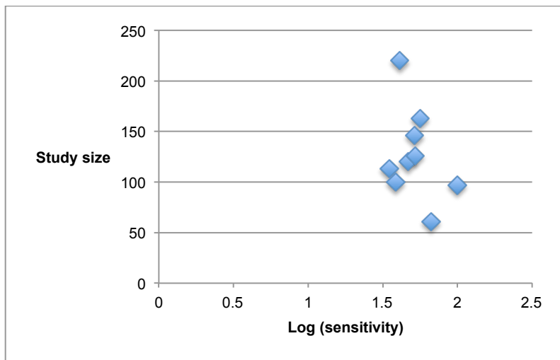
Appendix 4. Funnel plot of included studies demonstrating symmetrical scatter.
