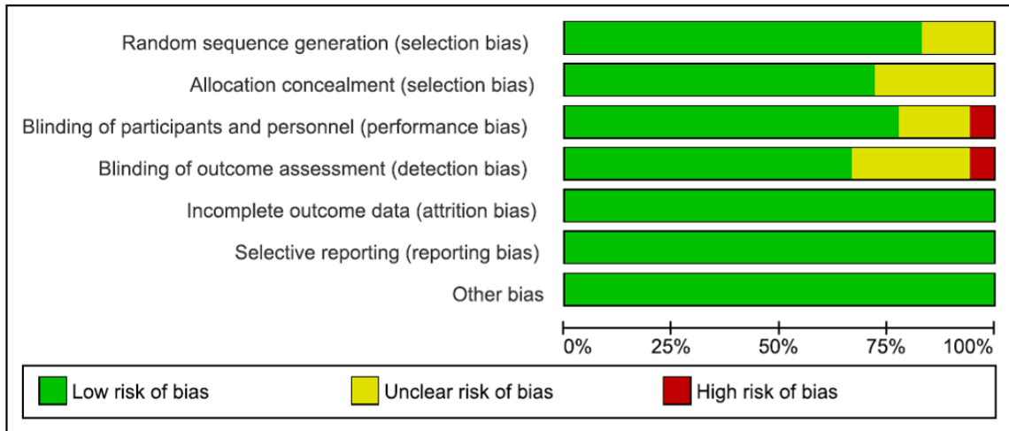
Supplement Figure 2. Risk of bias graph
