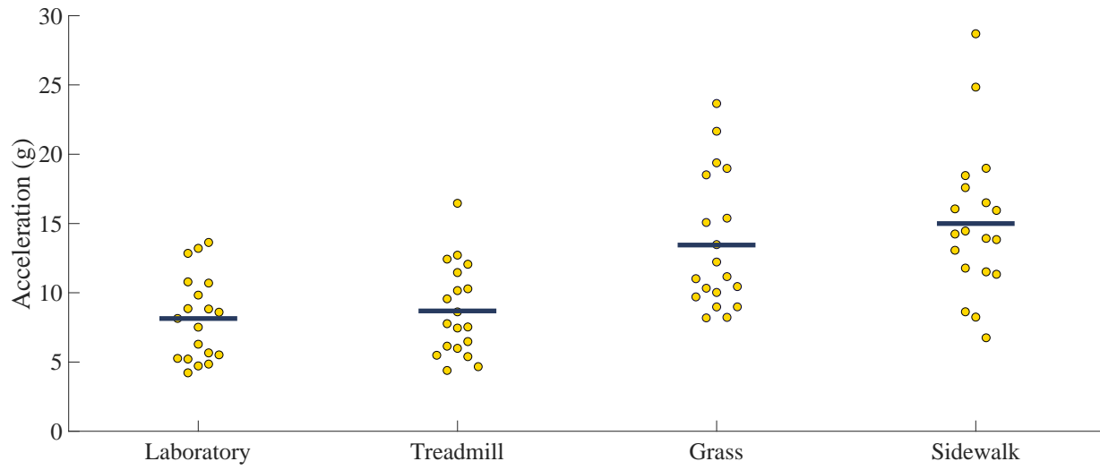
Supplemental Digital Content 2. Dot density plot of peak resultant tibial acceleration during overground, treadmill, grass, and sidewalk running. Each dot represents a single participant. The solid line represents the mean for each condition.
