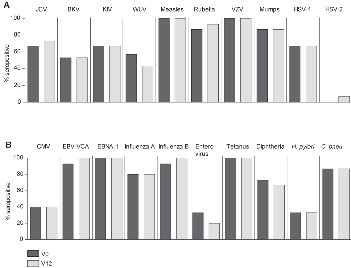
Figure e-1. Prevalence of MS patients seropositive for the depicted antigens before and during natalizumab treatment. (A and B) Prevalence of patients seropositive for antigens indicated, before (V0, dark grey bars) and after 12 months of natalizumab treatment (V12, light grey bars). Statistics: McNemar test (A and B).
