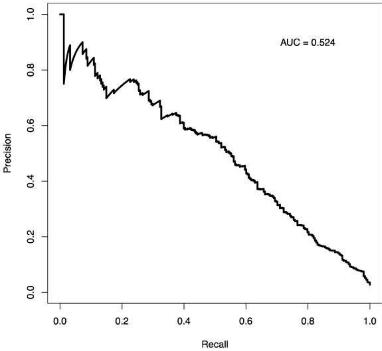
Precision Recall Curve
