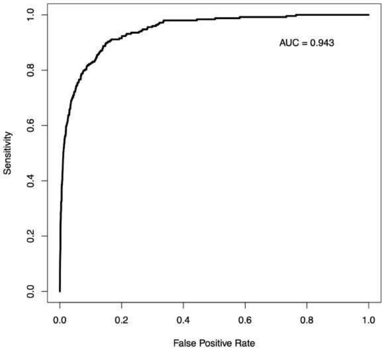
Supplemental Figure 3: PHIS+ Novel Mortality Score Performance. Panel S3A shows the receiver operating characteristic curve. Panel S3B shows the precision recall curve. The x-axis shows recall (sensitivity). The y-axis shows precision (positive predictive value). Panel S3C shows the GiViTI calibration belt. The p-value is a likelihood ratio test evaluating the deviation of the model from the observed result, a non-significant p-value is desirable. All panels show the model performance on the testing subset.
